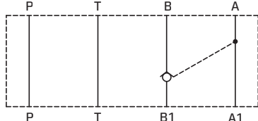
AM5-CP-B
