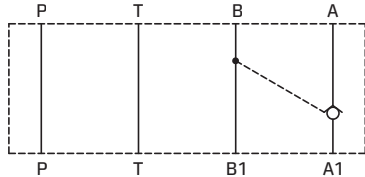
AM5-CP-B
